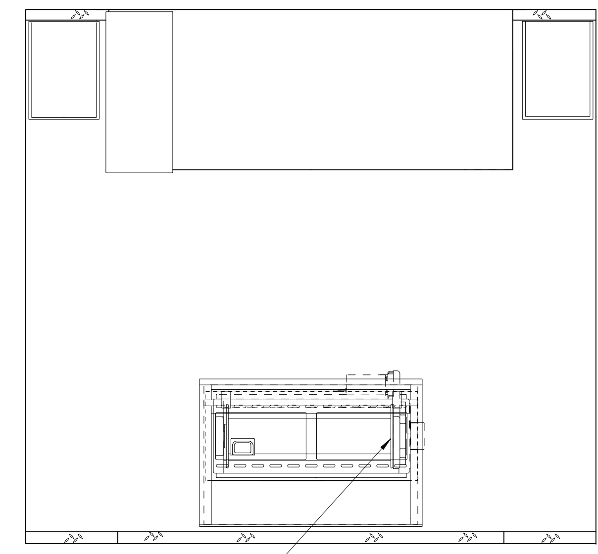
HANNAY ELECTRIC REWIND CORD REEL MODEL ELFCR1636-10-11-6 WITH 175' OF 10/4 CORD
